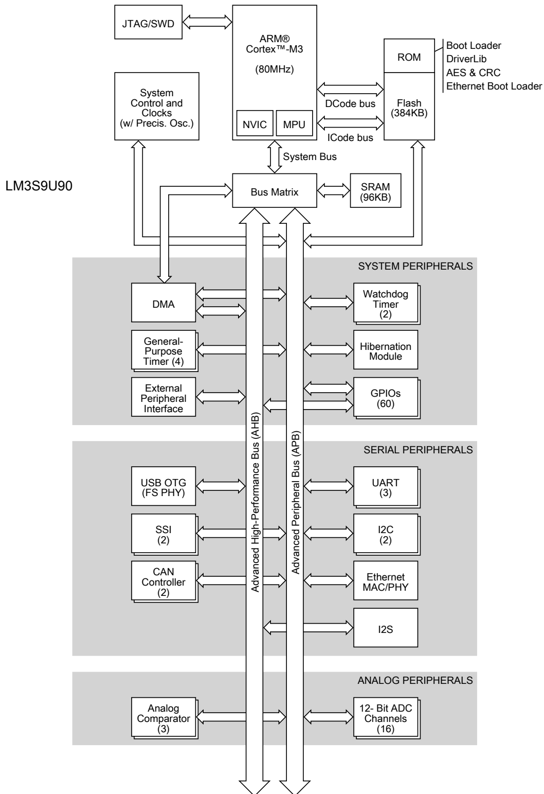
Figure 1-1. Stellaris LM3S9U90 Microcontroller High-Level Block Diagram
