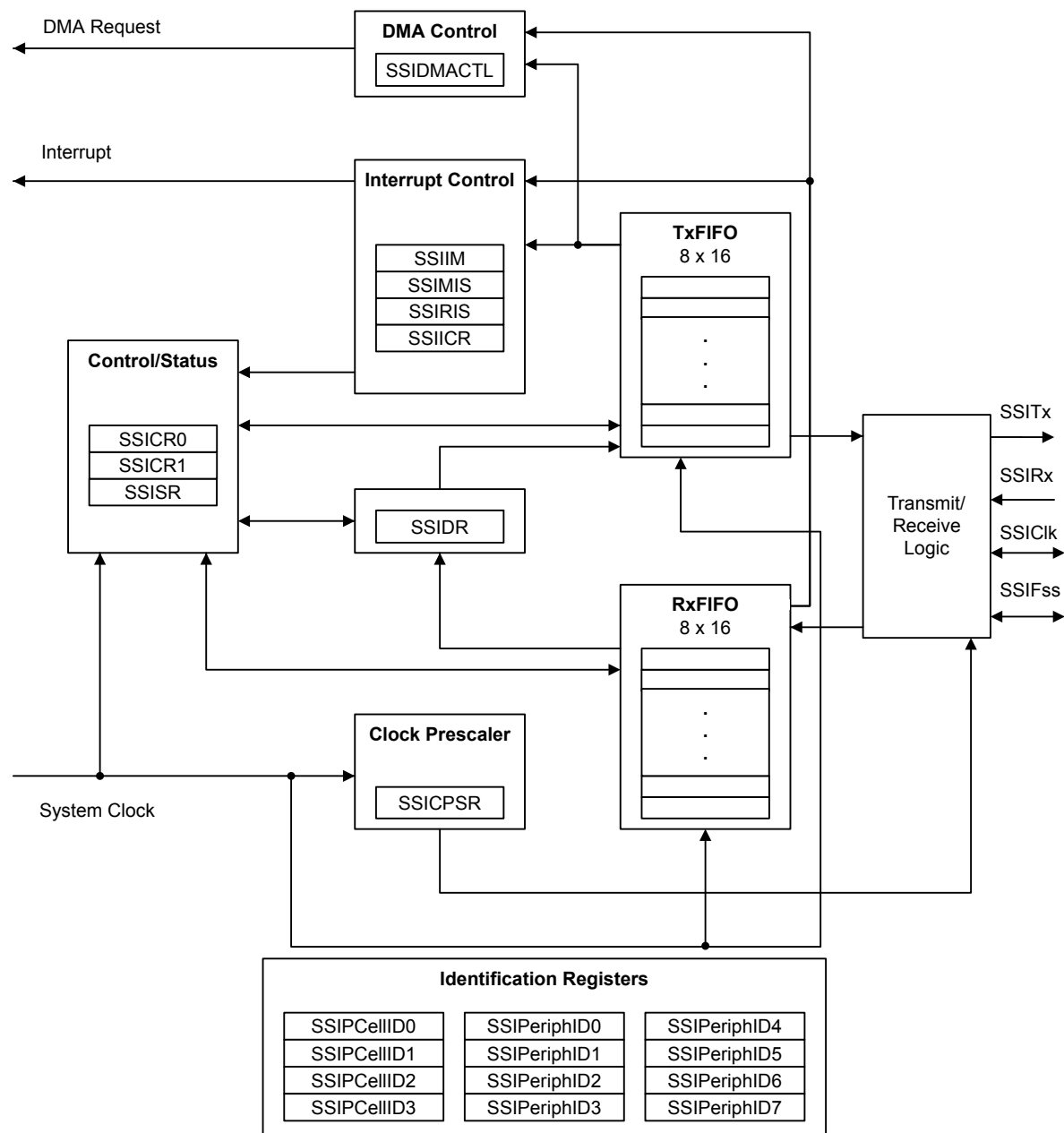
Figure 15-1. SSI Module Block Diagram
